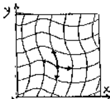
Fig 16. A NON-LINEAR 2-DIMENSIONAL GRID TENSOR FIELD.
