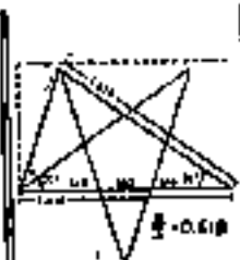
Fig 31. Origin of \Phi in 5-Point star.
